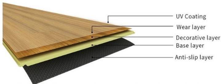
• SPC Structure
